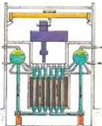
Steam-generating heavy-water reactor (SGHWR)
