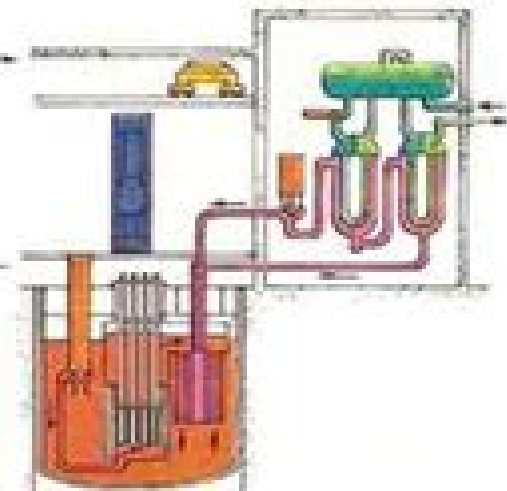
Fast breeder reactor (FBR)
