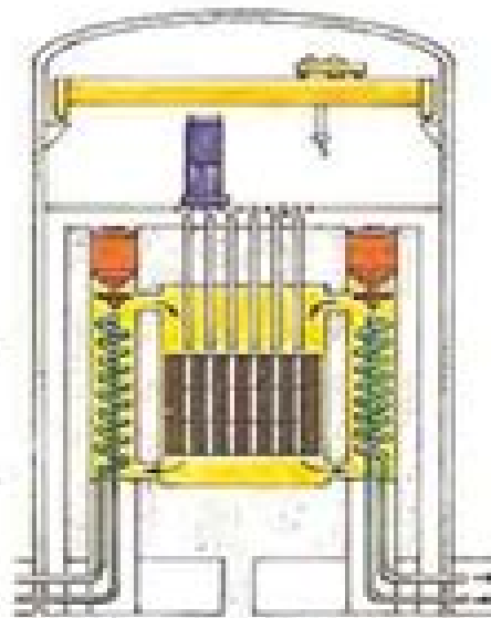
High-temperature graphite-moderated reactor (HTGR)
