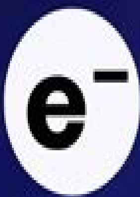
Electron
