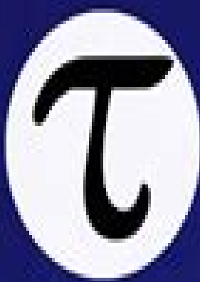
Tau
