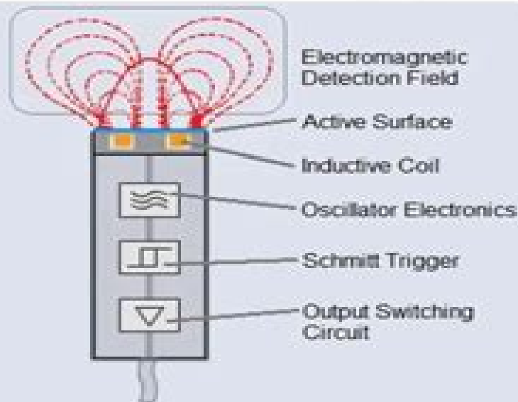
Internal Elements of an Inductive Proximity Sensor Source: automation-insights.blog
