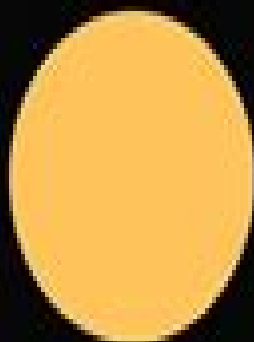
oval
