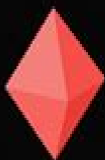
octahedron
