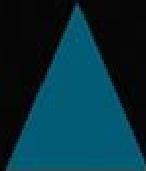
triangle
