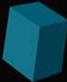
cube
