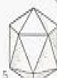
5 ICOSAEDRON (20 Triangles)
