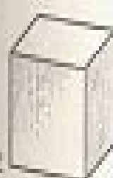
2 HEXAHEDRON (Cube)
