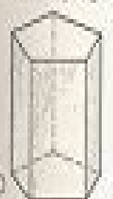
10 RIGHT PENTAGONAL
