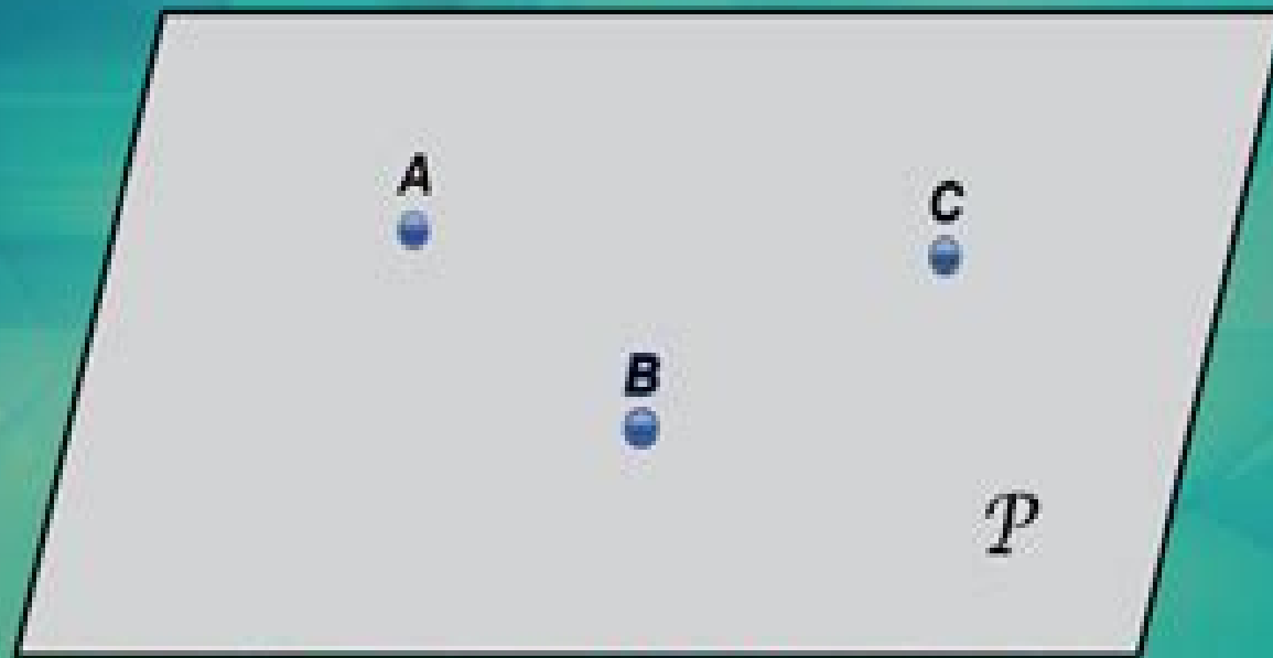
Plane \mathcal{P}
