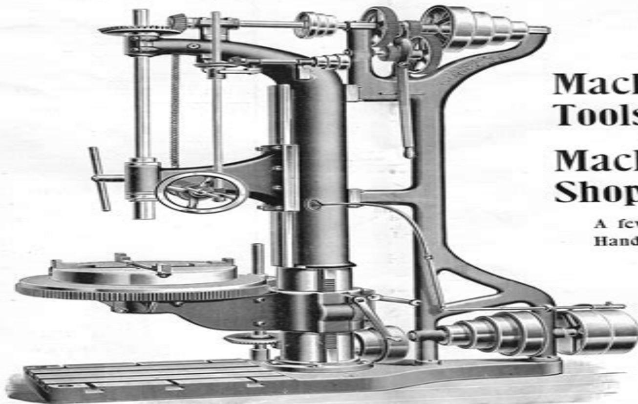
SNYDER 36-IN. STANDARD UPRIGHT DRILL. Back Geared, Automatic Feed, with Chucking Attachments.
