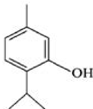
Thymol
