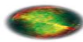
DUMBBELL NEBULA
