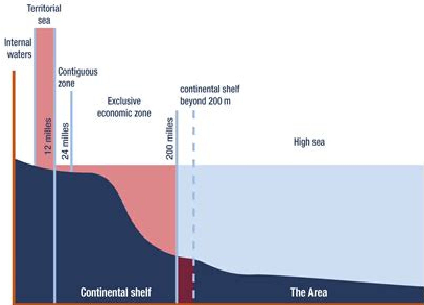
Scheme of maritime areas under jurisdiction of coastal States
