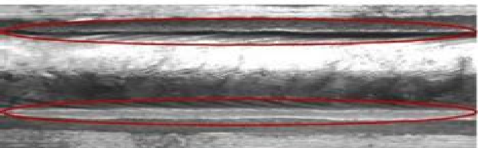
(c) Undercut
