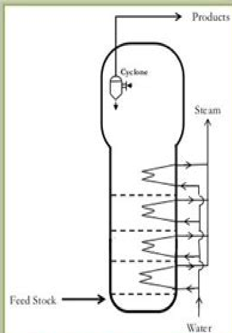
Fig: Reactor with a sectioned fluidized bed
