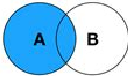
LEFT JOIN
