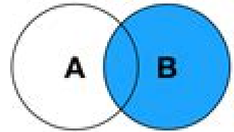
RIGHT JOIN
