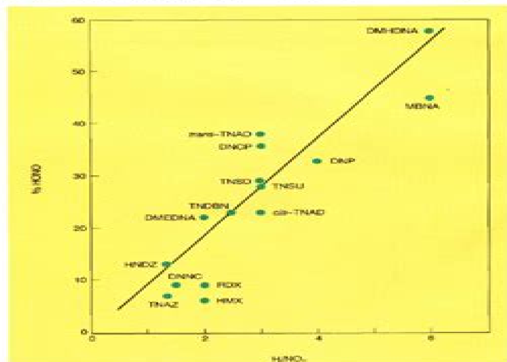
Figure 4. Plot of the initial relative percent concentration of HONO versus the H/NO 2 ratio in the parent molecule for a series of nitramine compounds.
