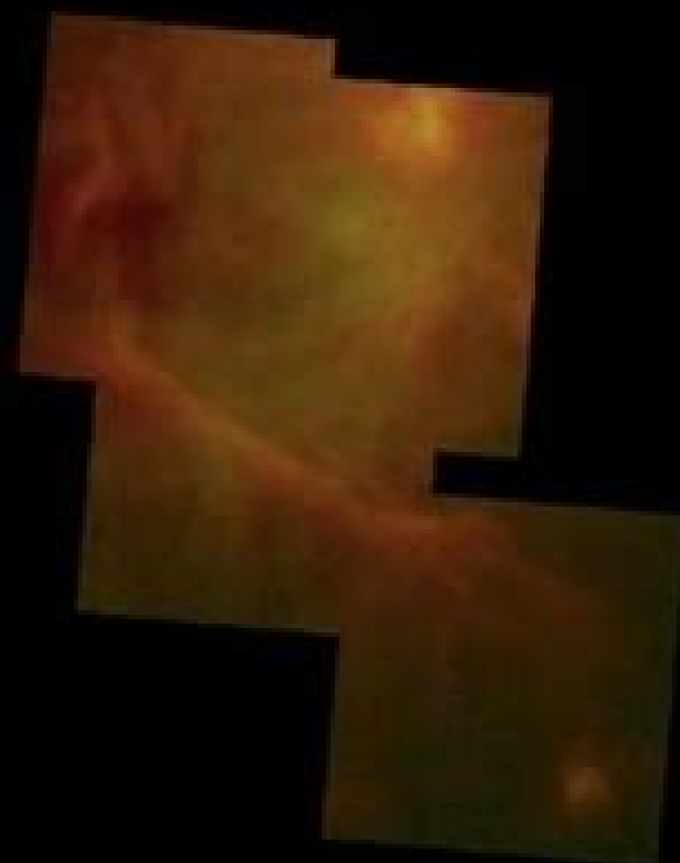
mid-infrared (SOFIA)
