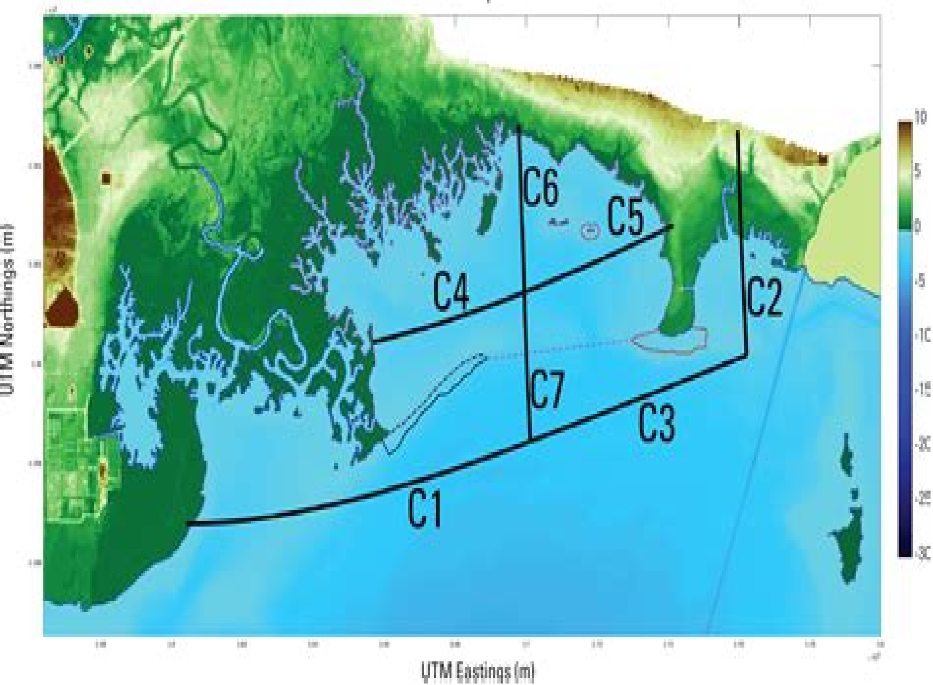
Observational Cross-Sections : Output locations of Sediment Fluxes
