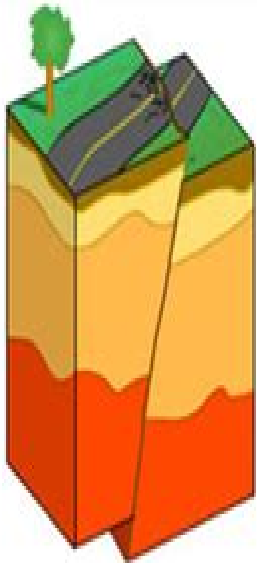
Reverse fault
