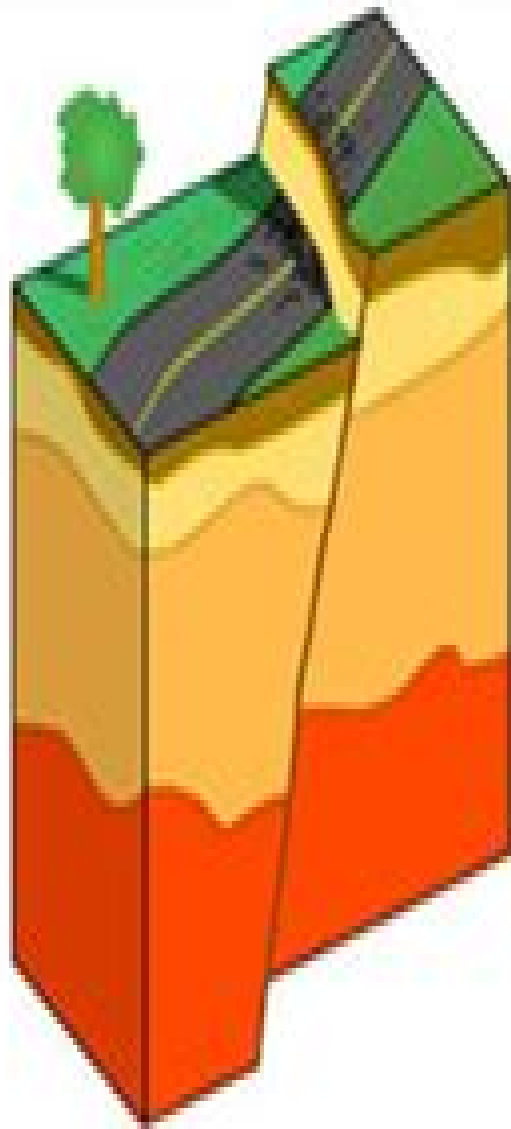
Normal fault
