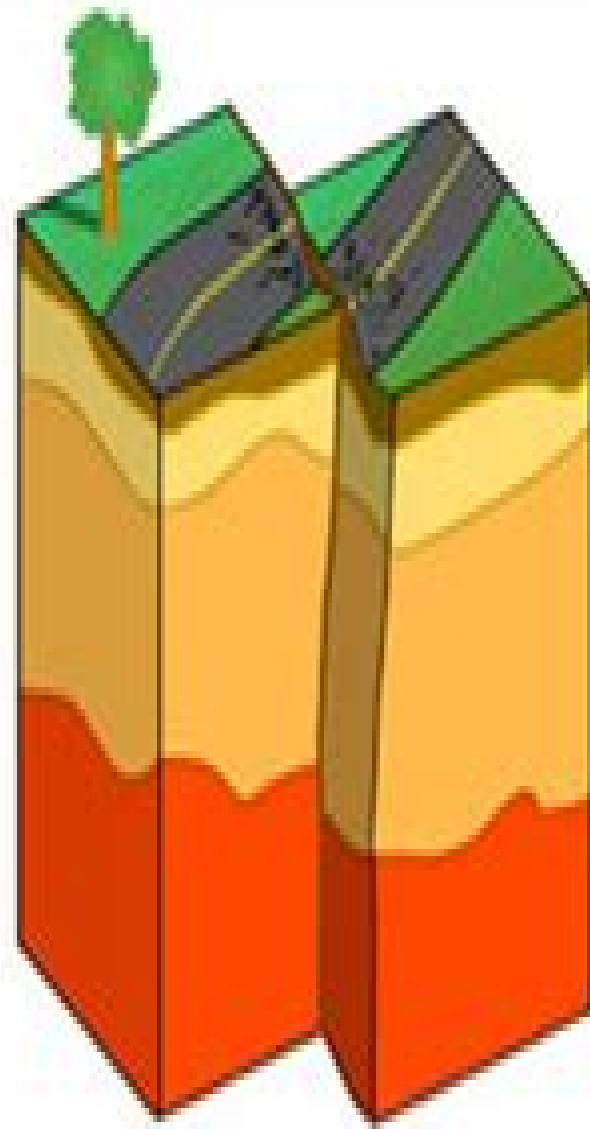
Strike-slip fault
