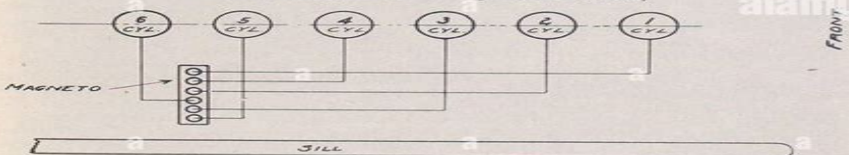
TO FIRE: 1-4-2-6-3-5. Wiring Diagram (Six-Cylinder Models)
