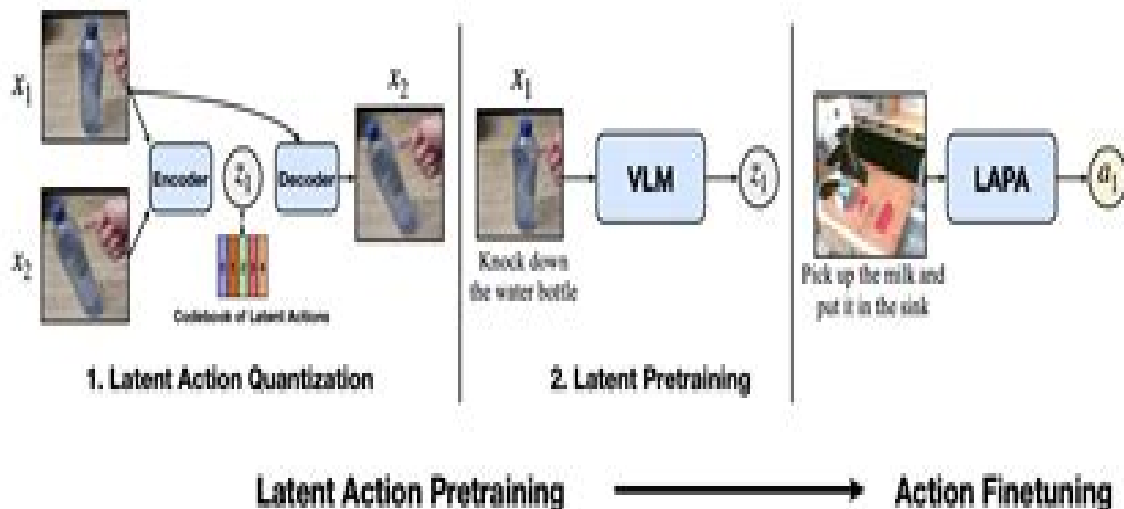
Figure 2: Overview of LAPA. (1) Latent Action Quantization: We first learn discrete latent actions in a fully unsupervised manner using the VQ-VAE objective. (2) Latent Pretraining: The VLM is trained to predict latent actions, essentially performing behavior cloning. After pretraining, we finetune the LAPA model on a small set of action-labeled trajectories to map the latent space to the end effector delta action space.
