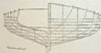
Fig. 4.16B Half plan and deck layout of Spruce
