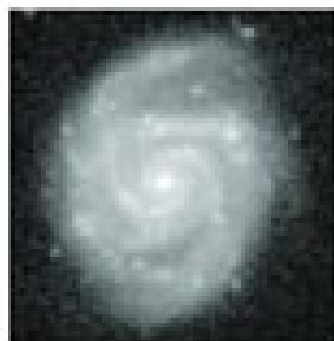
spiral (0.59)
