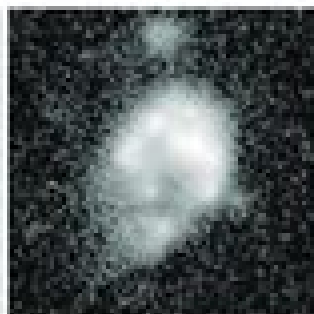
clump clusters (1.26)
