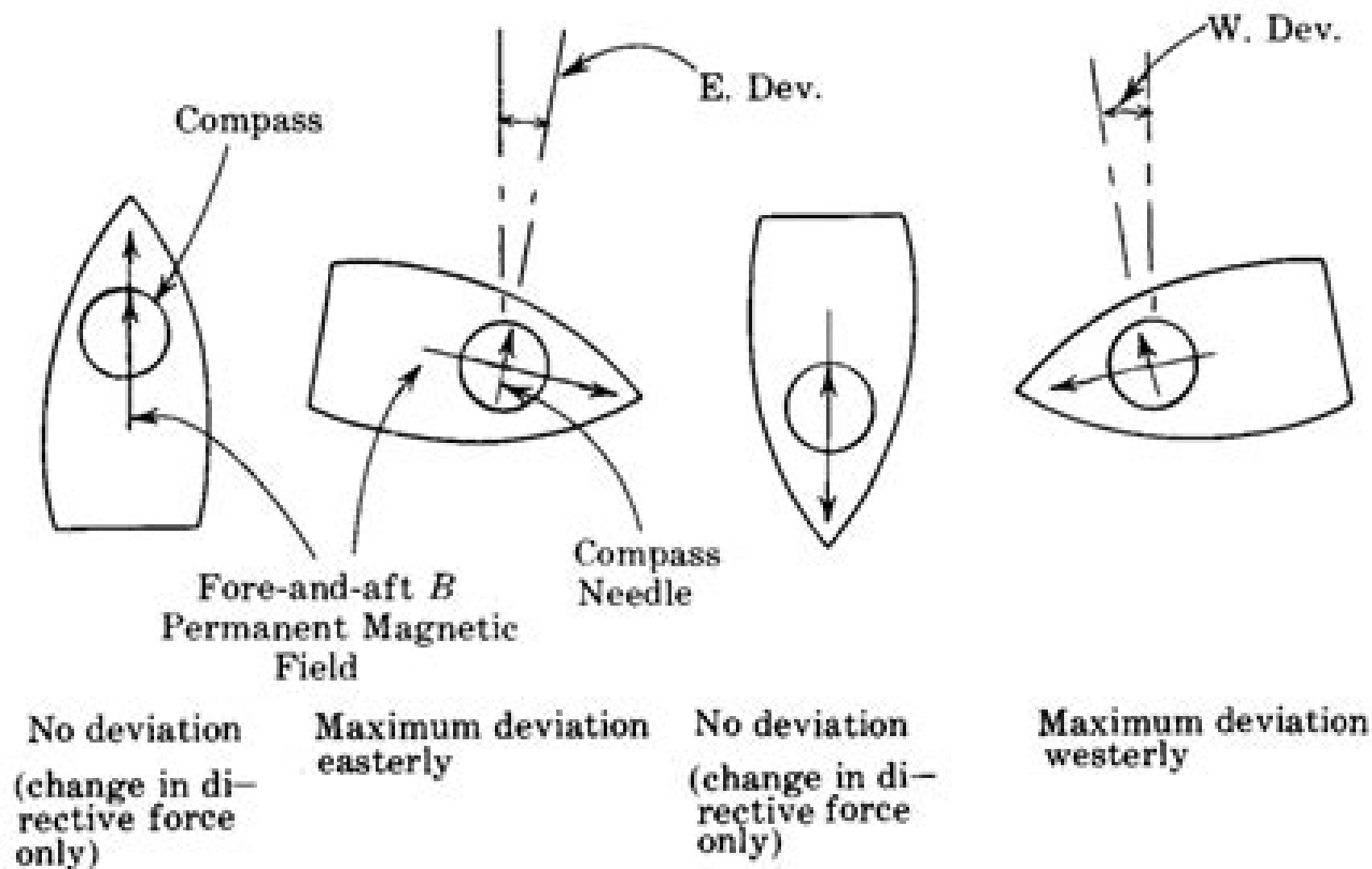
Figure 3 – Force diagrams for fore-and-aft permanent B magnetic field
