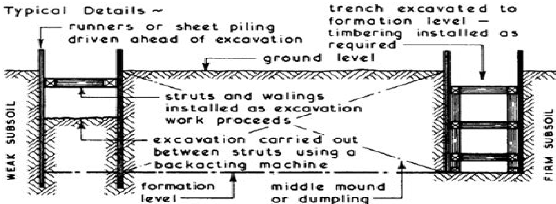
STAGE 1 - EXCAVATION OF PERIMETER TRENCH
