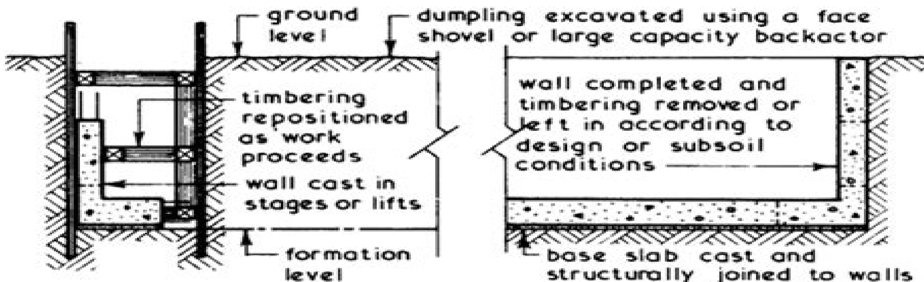
STAGE 2 - CONSTRUCTION OF BASEMENT WALLS
