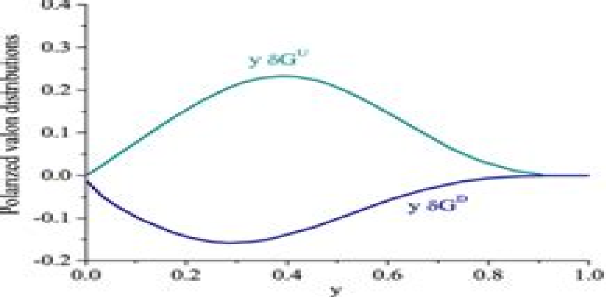
FIG. 1. (Color online): Polarized valon distribution functions for u and d valon types (the helicity distributions for the valons) inside a proton.
