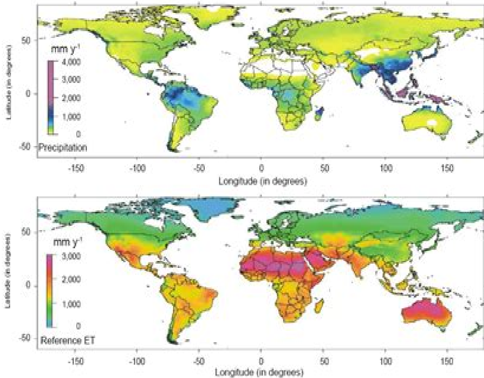
Figure 1: Annual global precipitation and reference evapotranspiration rates from IWM's Climate Atlas.
