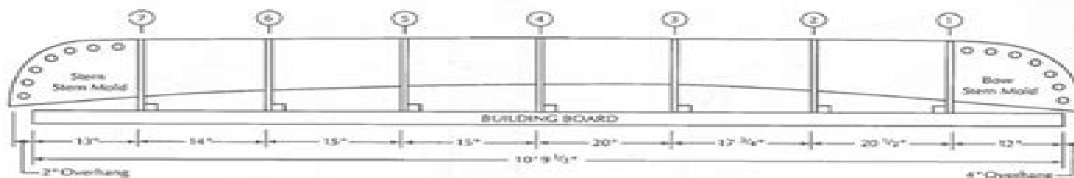
Bow Stem Mold (Not to scale)
