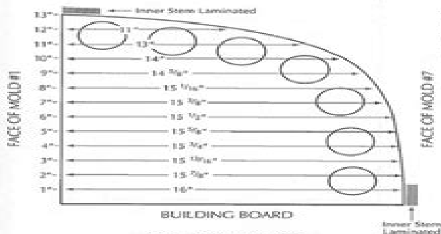
Bow Stem Mold (Not to scale)
