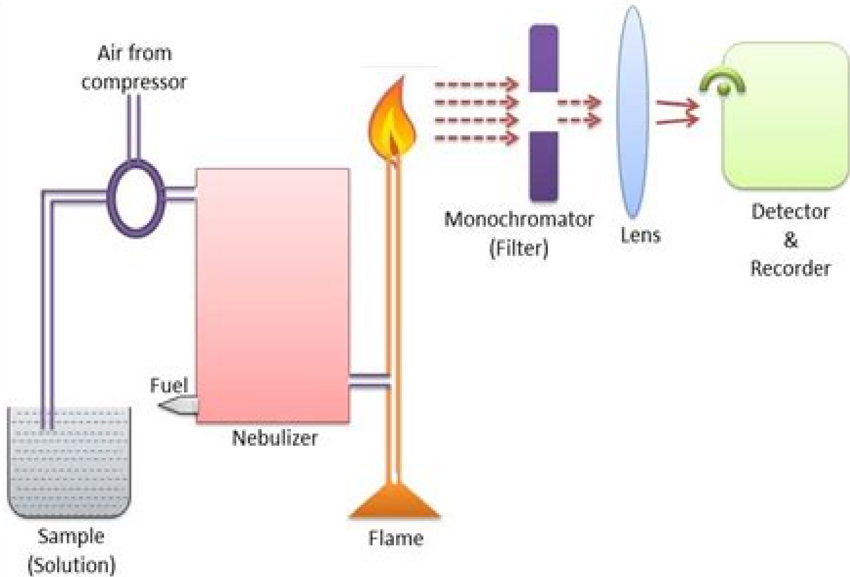
Instrumentation of Flame Photometer
