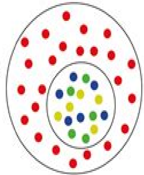
Integration
