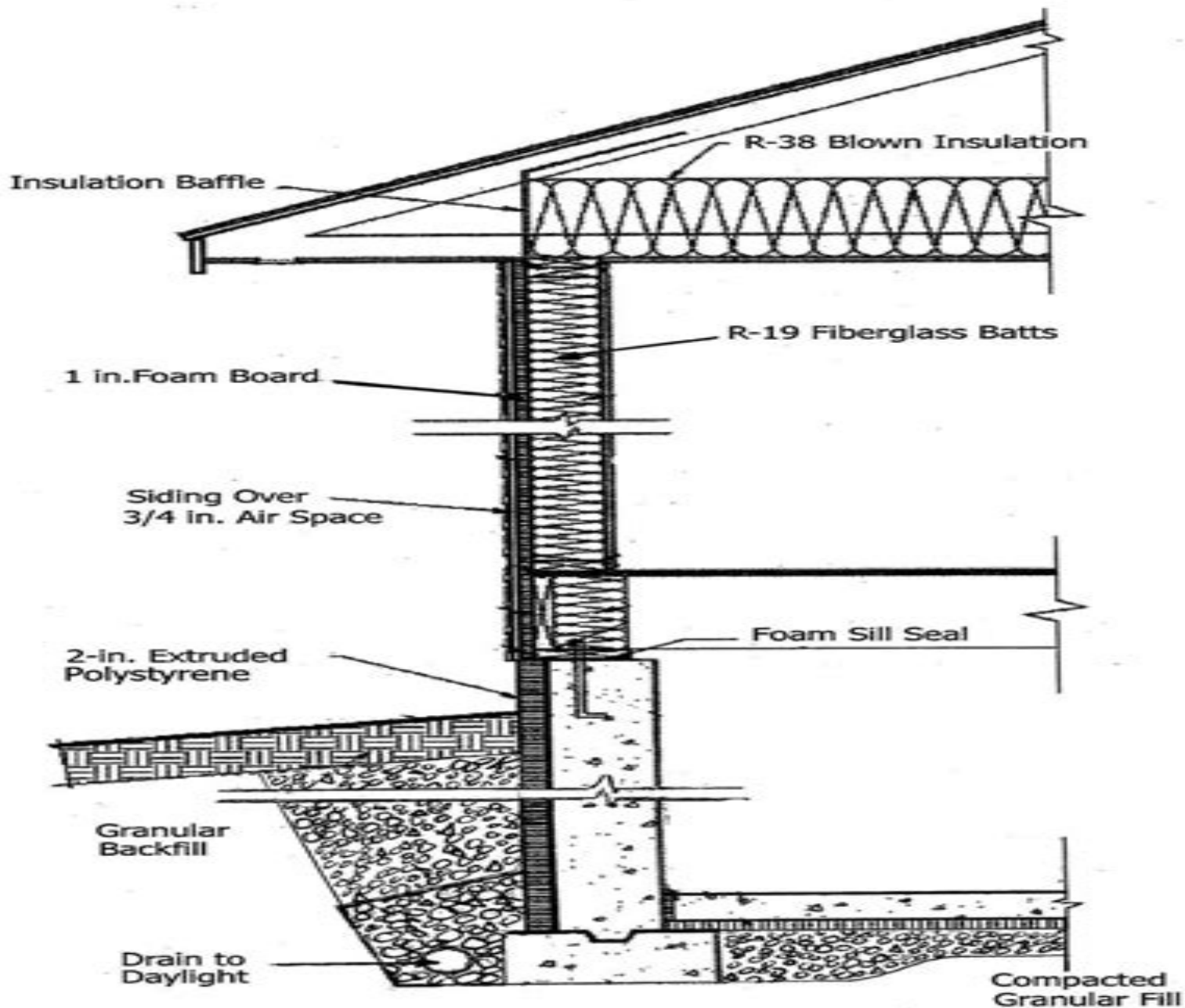
WALL SECTION - TYP.
