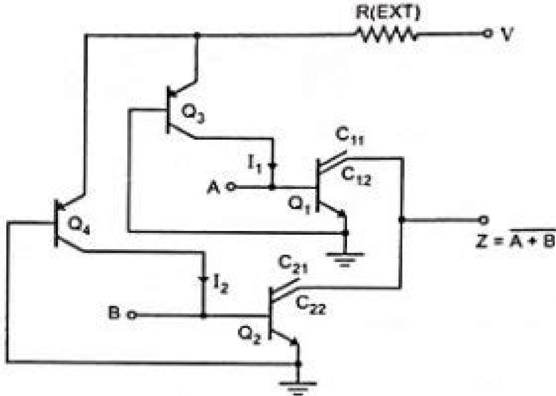
Fig. 47.7 IIL Logic NOR Gate
