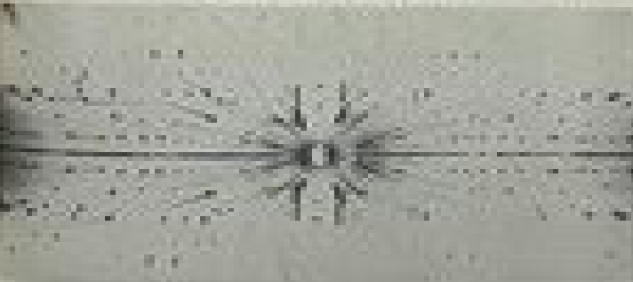
FIG. 12. DISTRIBUTION OF MATTER IN THE SOLAR SYSTEM
