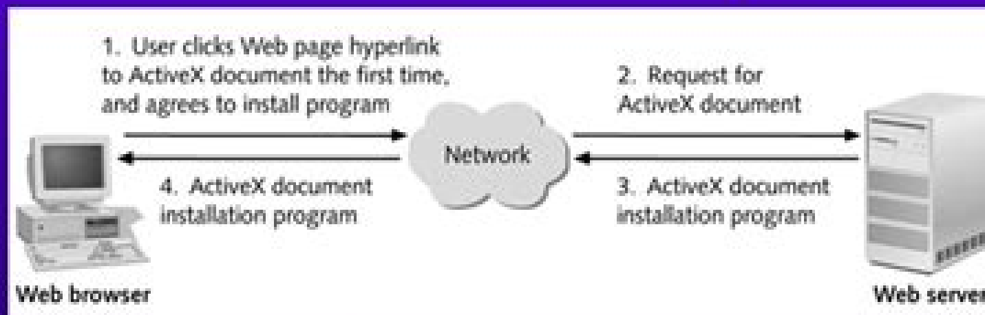
Figure 6-1: Installing an ActiveX document
